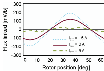
Fig. 8. Flux linked waveform for different values of DC field excitation current
