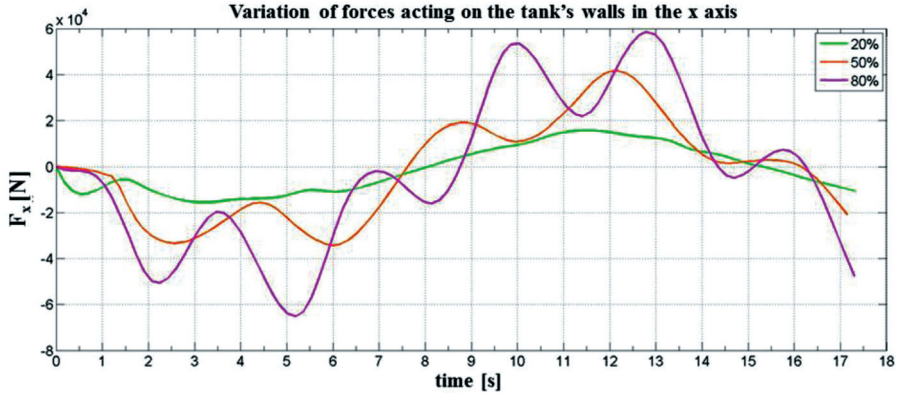
Fig. 18. Comparison of the unsteady forces acting on the tank wall in the direction along longer axis of the tank, for different tank filling level
