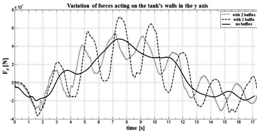
Fig. 28. Comparison of the unsteady forces acting on the tank wall in direction normal to longer axis of the tank, for different tank internal configuration
