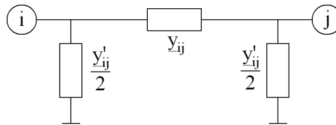
Fig. 1. Branch model in power system
