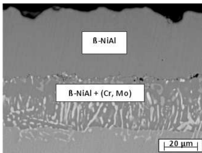
Fig. 3. The microstructure of aluminide layer deposited in the low-activity CVD process at the temperature 1050°C during 4h on Inconel 713 LC Ni-base superalloy
