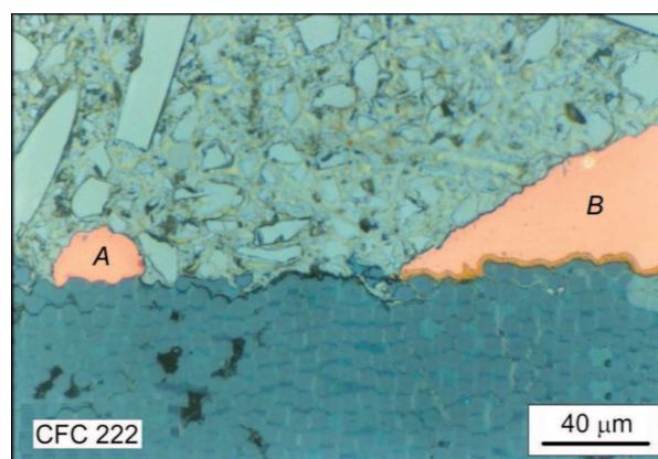
Fig. 6. Substrate of graphite composite CFC 222 wetted with two drops of CuCr1 brazing alloy
