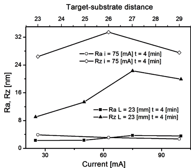
Fig. 5. Roughness of sputtered Cu layer using AFM for films deposited for a different current (area 5 \mu\text{m} \times 5 \mu\text{m} ) and for different target-substrate distance (area 10 \mu\text{m} \times 10 \mu\text{m} )
