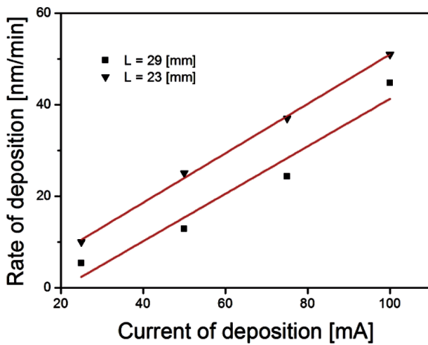
Fig. 3. Dependence between the current and the rate of deposition for different L values (L = target – substrate distance)
