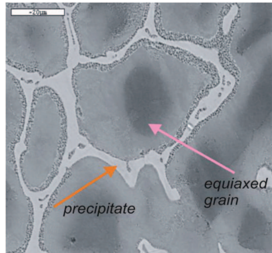
Fig. 21. Typical equiaxed structure containing a primary phase surrounded by a precipitate, [8]
