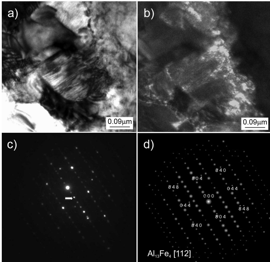
Fig. 6. TEM micrograph of the coating/substrate area. Bright field image (a), dark field image (b) at the ED reflex indicated by white arrow (c) and corresponding indexed simulation of the \text{FeAl}_3 ( \text{Fe}_4\text{Al}_{13} ) diffraction (d). Atoms unit cell coordinates taken from the reference [12]
