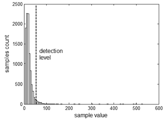
Fig. 11. Sample histogram after amplitude detection. Peak detection level is shown.
