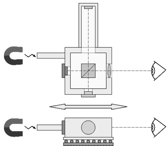
Fig. 4. Experimental pachymeter. Side view shows ball bearing. Magnetic drive is shown schematically.
