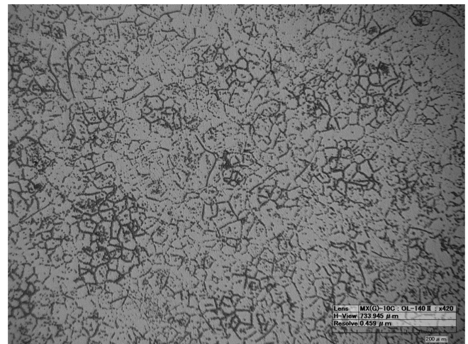
Fig. 4. Digital microscopic structure of the cold drawn and solution treated and aged sample exhibiting \alpha precipitates (dark) in \beta grains
