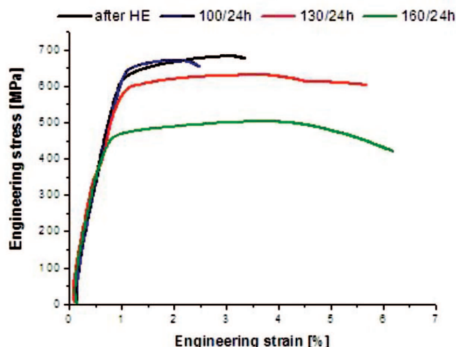
Fig. 2. The comparison of the tensile curves of a nanograined aluminium alloy aged at 100, 130 and 160°C for 24 hours
