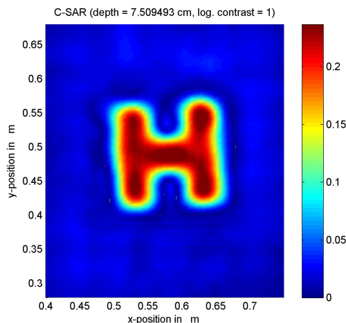
Fig. 11. SAR focussed radarscan of H-shaped object with 10cm focal radius.
