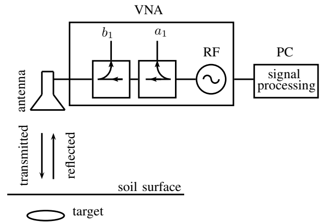
Fig. 4. GPR system model for a monostatic instrumentation setup.
