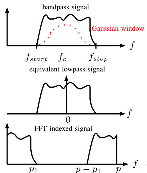
Fig. 6. Signal-processing of radar raw data.
