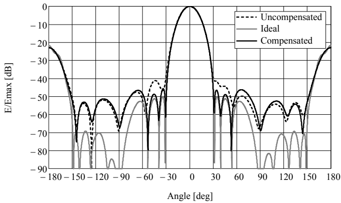
Fig. 12. Comparison of ideal, uncompensated and compensated radiation patterns of the antenna array for d_p = 0.1\lambda_0 and SLL = -50 dB.
