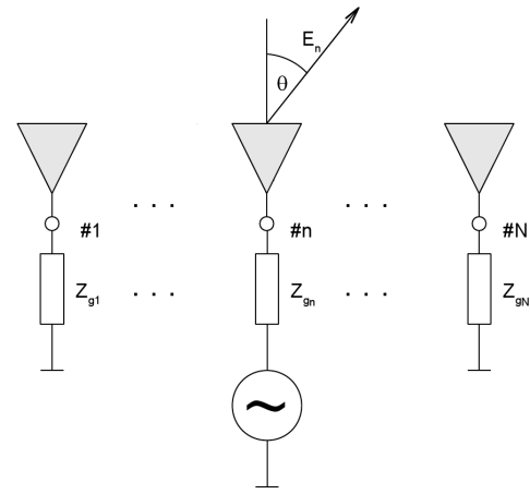
Fig. 2. Geometry for determination of the active element radiation pattern.
