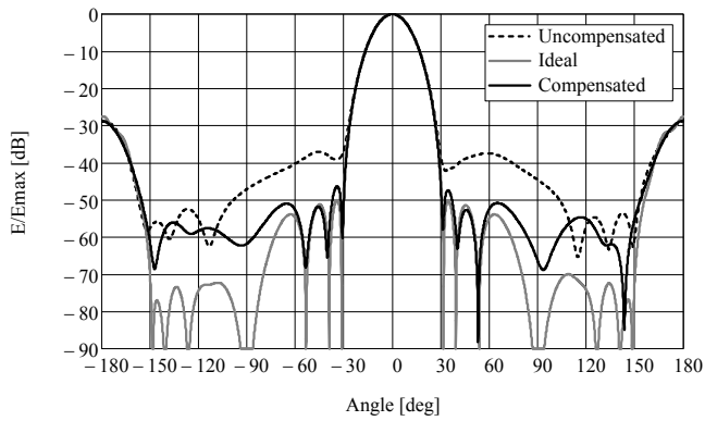
Fig. 11. Comparison of ideal, uncompensated and compensated radiation patterns of the antenna array for d_p = 0.25\lambda_0 and SLL = -50 dB.
