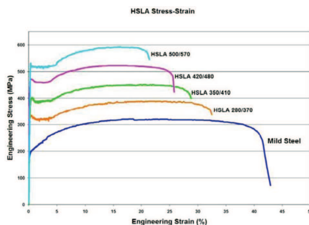
Fig. 3. Tensile stress-strain curves of various HSLA steels compared with mild steel
