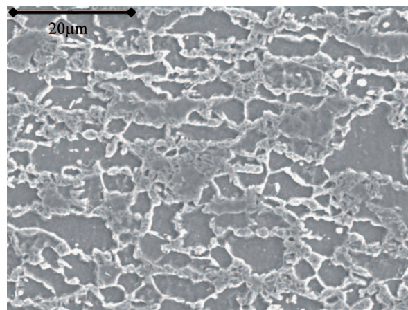
Fig. 11. Microstructure of DP600 base material, etched with 5-% nital, SEM
