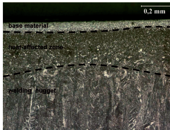
Fig. 12. Microstructure of DP600 weld: base material, heat-affected zone and weld nugget, etched with 5-% nital, light microscope
