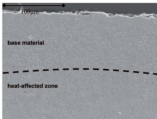
Fig. 7. Microstructure of HSLA340 weld: base material and heat-affected zone on the electrode side, etched with 5-% nital, SEM
