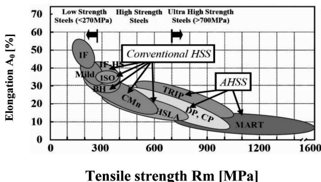
Fig. 1. Relationship between elongation and tensile strength of various steels used in automotive industry [6]
