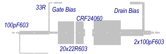
Fig. 7. The single amplifier layout with CRF24060 SiC MESFET (substrate: RT/Duroid \epsilon_r=10.2 h=1.27mm, t=35 \mu m).
