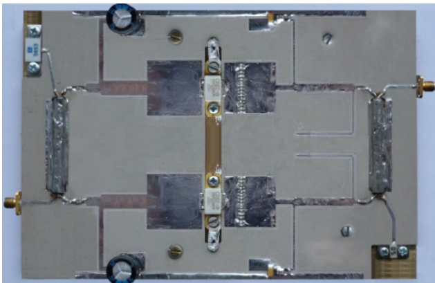
Fig. 10. The photo of of the balanced amplifier with CRF24060 SiC MESFETs.
