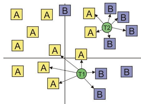
Fig. 3. An example of k-NN classification. Test samples (marked described T_1 and T_2 ) should be assigned to the first class A or to the second class B, which is determined based on calculation of the distance between individual test samples and the representatives of two aforementioned classes. This value is dependent on the number of neighbors considered in calculations (the k value).
