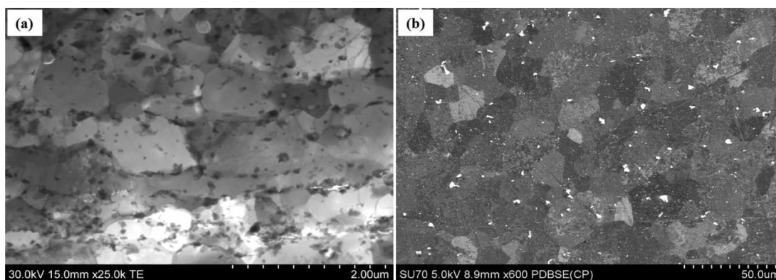
Fig. 1. SEM images of the 5083 alloy prepared by different processing routes: a) structure of RS material obtained by means of TE detector, b) structure of IM material obtained by BSE detector
