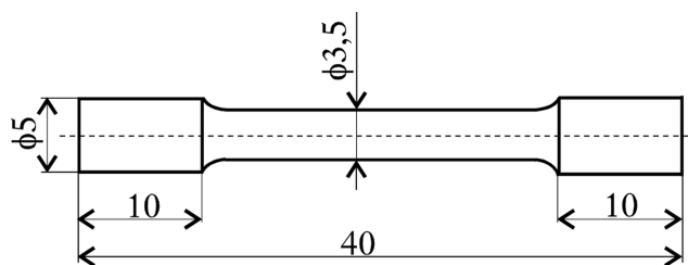
Fig. 2. Dimensions of the samples used in tensile strength tests
