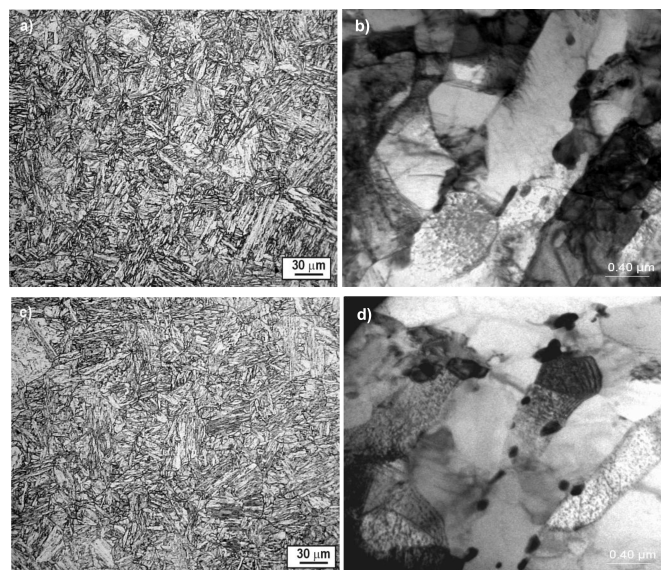
Fig. 6. Microstructure of GP91 cast steel after heat treatment: a, b) treatment No. 1; c, d) treatment No. 2; OM (a, c), TEM (b, d) – thin foil
