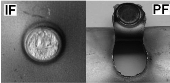
Fig. 4. Typical observed failure mode
