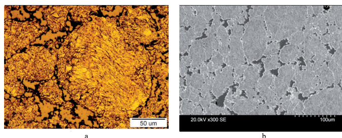
Fig. 5. Microstructure of AgNi consolidated by CEC, a) optical microscopy observation after 2 CEC cycles ( \phi = 0.84 ), b) SEM observation after the 4 CEC cycles ( \phi = 1.7 )
