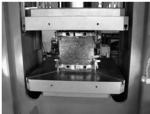
Fig. 1. A set of tools for die forging on a 2.5MN press – assembled
