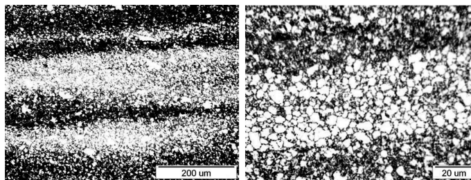
Fig. 13. Microstructure obtained in the forging process carried out at 400°C with the following heat-treatment to the T5 condition; examinations by light microscopy
