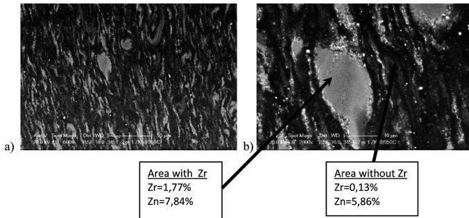
Fig. 6. SEM microstructure of ZK60A alloy forged at 400°C, T5 temper (a – mag. \times 500 , b – mag. \times 2000 ) with the EDS chemical analysis in microregions
