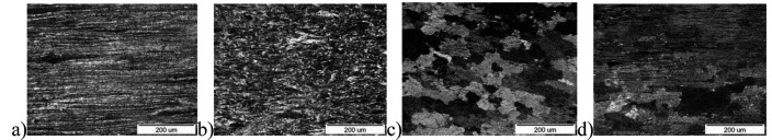
Fig. 9. Microstructures showing the grain size in ZK60A alloy forged at 350°C and heat treated to various conditions, a) T5 – non-recrystallised structure, b) T5 partially recrystallised structure, c) T6 (solutioning at 430°C) – completely recrystallised structure, d) T6 with local large grain size variations
