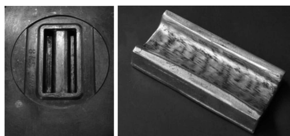
Fig. 3. Die insert to forge a flat model shape and flat model shape forged from magnesium alloy
