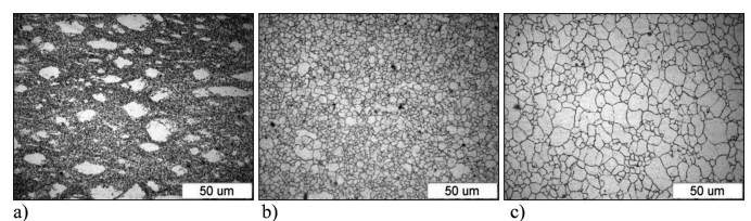
Fig. 8. Microstructure of AZ61 alloy after compression with strain rate of 0.1 to deformation \epsilon = 0.8 . Deformation temperature: a – 250°C, b – 300°C, c – 350°C
