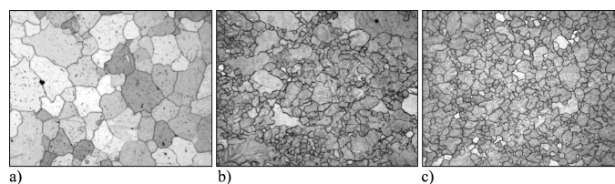
Fig. 4. The microstructure of the investigated AZ31 alloy after compression at a temperature of and 350°C – slip dominates. Strain rate of 0.1 s -1 , strain \epsilon : a – 0.1, b – 0.4, c – 0.8
