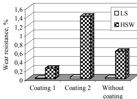
Fig. 5. Wear resistance of protective coatings
