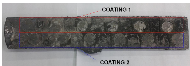
Fig. 8. Casting after being knocked-out – from the side of shaped samples with protective coatings
