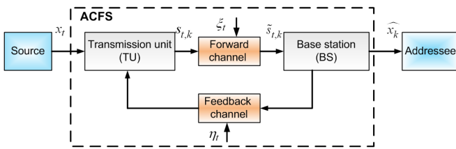
Fig. 1. A basic simplified block diagram of the AFCS. x_l -input signal, x_k -estimates of the input signal, \eta -noise in the forward and feedback channels, s -signals transmitted and received in the forward channel. Forward and Feedback channels may be RF, open optical or cable – fiber optic.
