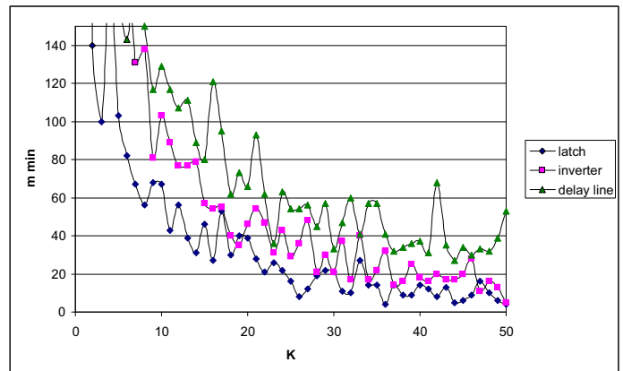
Fig. 8. The values of m_{min} for RBGs from Fig. 2 and three realizations of the delay \tau , f_L = 200 MHz.
