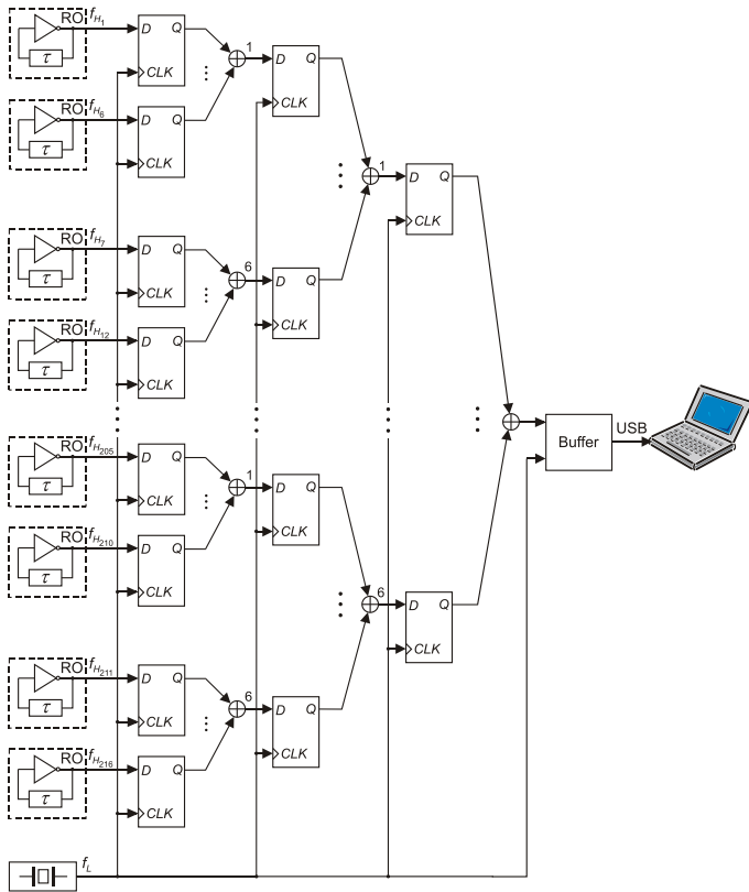
Fig. 2. Combined RO-based RBG.
