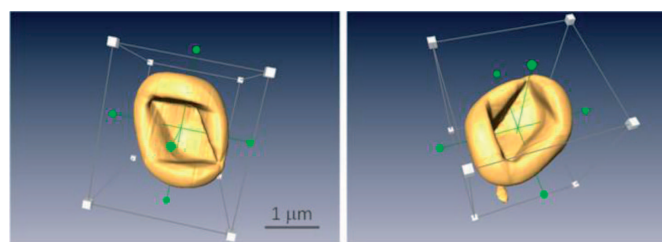
Fig. 6. 3D visualization of \text{Ti}(\text{C},\text{N}) particle
