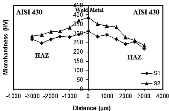
Fig. 6. Microhardness graphics of S1 and S2 specimens
