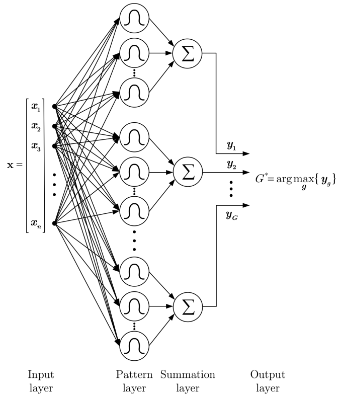
Fig. 1. The structure of the probabilistic neural network.
