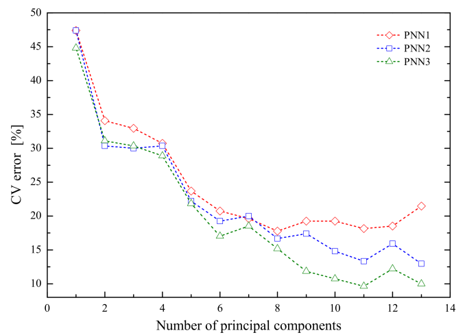
Fig. 11. Plot of the 10-fold cross validation error determined in relation to the number of principal components for SH data classification problem.
