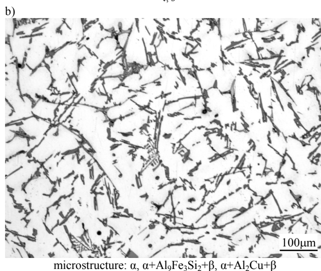
Fig. 1 (a, b). Representative TDA curves (a) and the microstructure (b) of 226 silumin after holding at a temperature of 680°C
