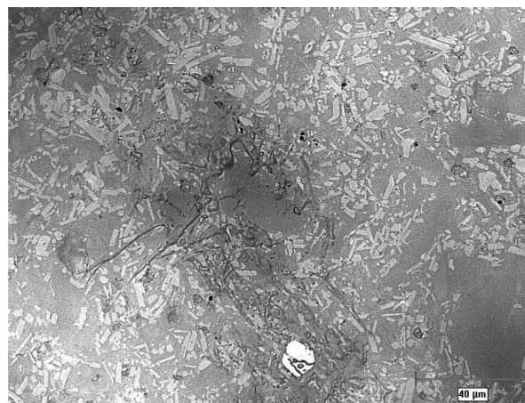
Fig. 8. Cracks in the mullite precipitate, propagating into the matrix, magnification 500 times. The structure of small size sample of C 130 material loaded up to the advanced subcritical stage
