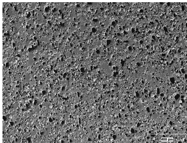
Fig. 4. The structure of C 120 type material of the rod of the long rod high voltage insulator of 1974, magnification 50 times. Advanced ageing processes are visible. More than 1/3 quartz grains was separated from the matrix and crushed out. Numerous fine cracks of the matrix are visible in their vicinity
