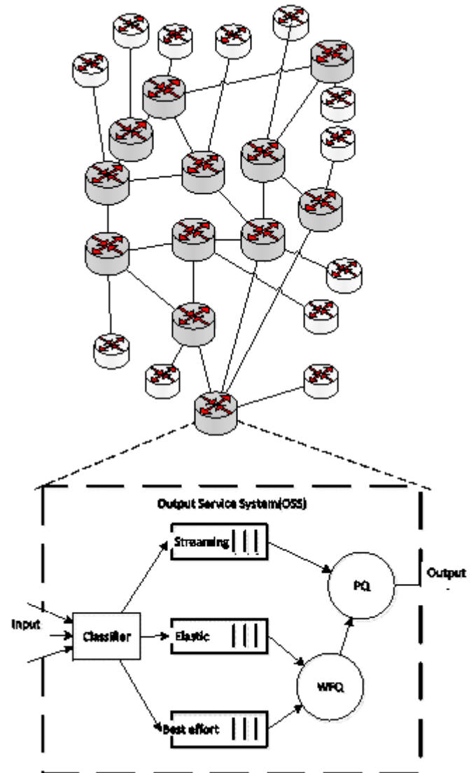
Fig. 1. Architecture of output service system.
