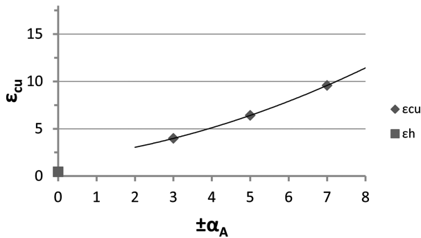
Fig. 20. Values of the cumulative strain \varepsilon_{cu} in function of the reverse torsion angle \pm\alpha_A ( f=0.71 [Hz], \nu=0.1 [mm/s], \varepsilon_h \approx 0.45 at the value of draft as in case of the unconstrained compression test)
