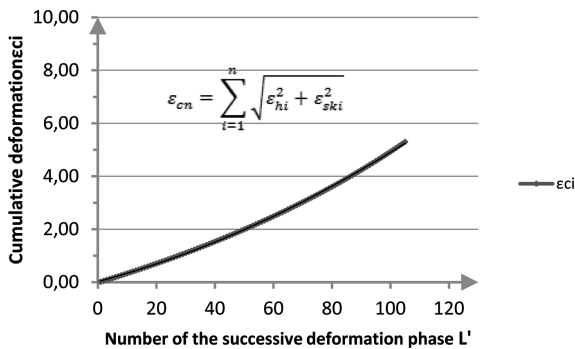
Fig. 17.b. Change of the values of the cumulative strain \epsilon_{ci} during the successive deformation phases (the conditions for the reversible motion of the punches \alpha_A = \pm 3^\circ , f=1 [Hz])
