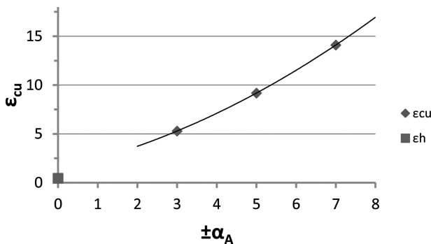
Fig. 21. Values of the cumulative strain \varepsilon_{cu} in function of the reverse torsion angle \pm\alpha_A (sinters having the initial density, f=1,0 [Hz], \nu=0.1 [mm/s], \varepsilon_h \approx 0.45 at the value of draft as in case of the unconstrained compression test)
