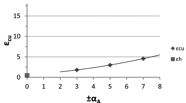
Fig. 19. Values of the cumulative strain \epsilon_{cu} in function of the reverse torsion angle \pm\alpha_A ( f=0.32 [Hz], v=0.1 [mm/s], \epsilon_h \approx 0.45 at the value of draft as in case of the unconstrained compression test)
