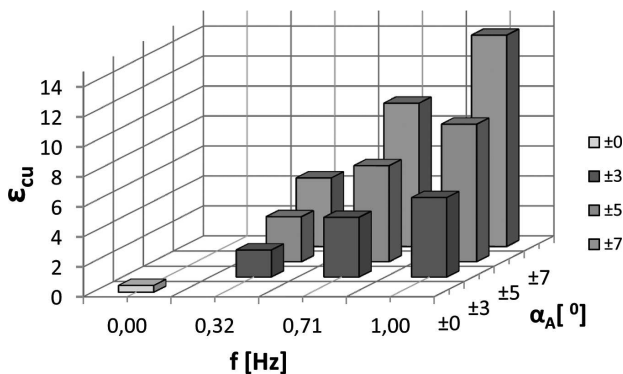
Fig. 22. Values of the cumulative strain \varepsilon_{cu} in function of the reverse torsion angle \pm\alpha_A and the torsion cycle frequency f ( \nu=0.1 [mm/s], \varepsilon_h \approx 0.45 at the value of draft as in case of the unconstrained compression test)
