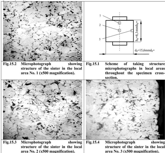
Fig. 15. Metallographic images of the structures in local areas of sintered iron (NC100.24) for the situations after deformation under combined load conditions (average relative density prior to deformation \rho_w = 0.75 , deformation conditions: oscillatory torsion angle \alpha_A = \pm 5^\circ , compression velocity v = 0.1 [mm/s], cycle frequency f = 0.71 [Hz], test specimen No. 1.2.1., average density of the sinter after deformation \rho_w = 0.97 , average porosity of the sinter after deformation \phi = 3\% )
