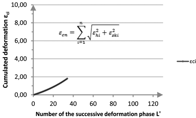
Fig. 16.b. Change of the values of the cumulative strain \epsilon_{ci} during the successive deformation phases (the conditions for the reversible motion of the punches \alpha_A = \pm 3^\circ , f=0.32 [Hz])
