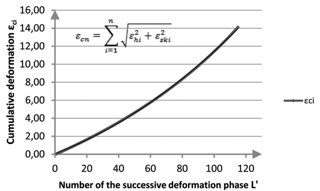
Fig. 18.b. Change of the values of the cumulative strain \epsilon_{ci} during the successive deformation phases (the conditions for the reversible motion of the punches \alpha_A = \pm 7^\circ , f=1,0 [Hz])
