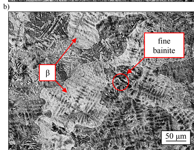
Fig. 10. Microstructure in the granule of CuAl10Fe5Ni5 bronze (a,b), E_3(1180,116)
