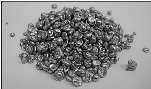
Fig. 3. Granules of CuAl10Fe5Ni5 bronze cast on INDUTHERM-VC 500 D Vacuum Pressure Casting Machine according to the plan of the experiment E_3(1180.116)
