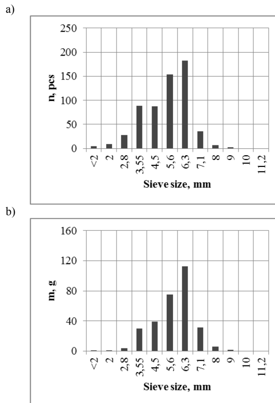
Fig. 8. Number of granules n in mesh fraction (a) and weight m granules weight on sieve (b); E_3(1180,116)
