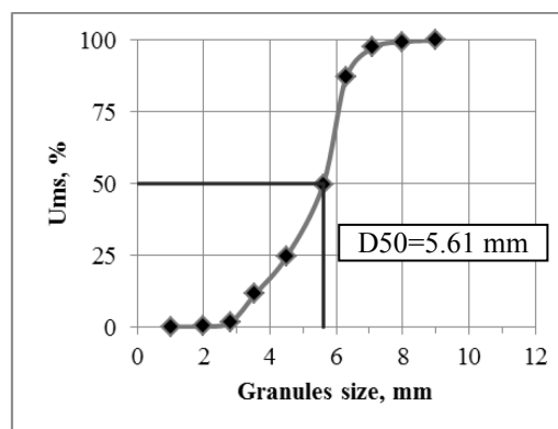
Fig. 9. Curve of cumulative percent retained "Ums" in % of mesh fraction for granulates of CuAl10Fe5Ni5 bronze; E_3(1180,116)
