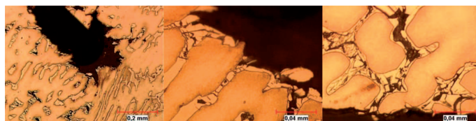
Fig. 4. Microstructure of specimen made of LH556 cast alloy after the perforation test
