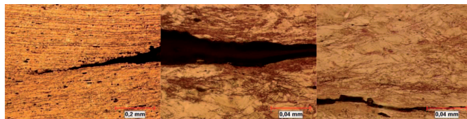
Fig. 3. Microstructure of specimen made of VP 159 steel after the perforation test
