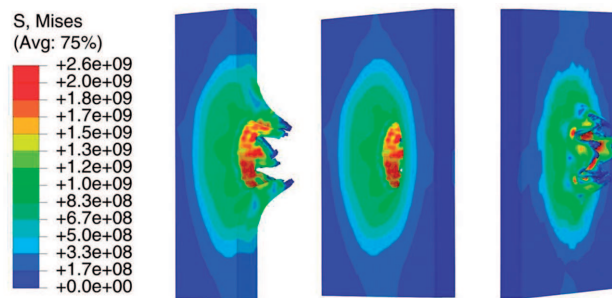
Fig. 10. Results of FEM simulation of VP159 steel perforation tests
