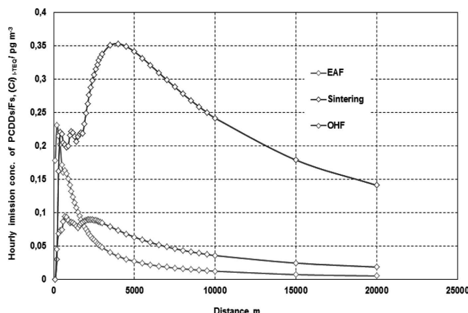
Fig. 3. Dependence of the hourly imission concentration profiles ( C t ) PCDDs/Fs on the distance from the source in the year with the highest total emission (1989)
