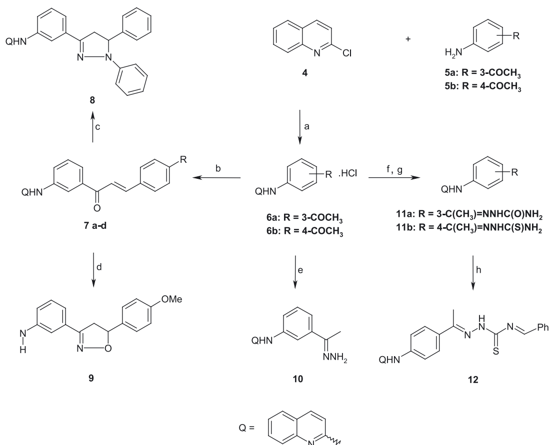
Fig. 2. Reagents and conditions: (a) EtOH, HCl, rfx., 70% for 6a; (b) PhCHO, NaOH, EtOH, 7a (65%), p -MeOC 6 H 4 CHO, NaOH, EtOH 7b (70%), p -ClC 6 H 4 CHO, NaOH, EtOH 7c (60%), m -HOC 6 H 4 CHO, NaOH, EtOH 7d (75%); (c) 7a, PhNHNH 2 , EtOH, rfx., 60%; (d) 7b, NH 2 OH.HCl, NaOH, EtOH, rfx., 70%; (e) N 2 H 4 , H 2 O, H 2 SO 4 , 80%; (f) 6a, Semicarbazide, EtOH, rfx., 65%; (g) 6b, Thiosemicarbazide, EtOH, rfx., 60%; (h) 11b, BzH, EtOH, rfx., 65%
