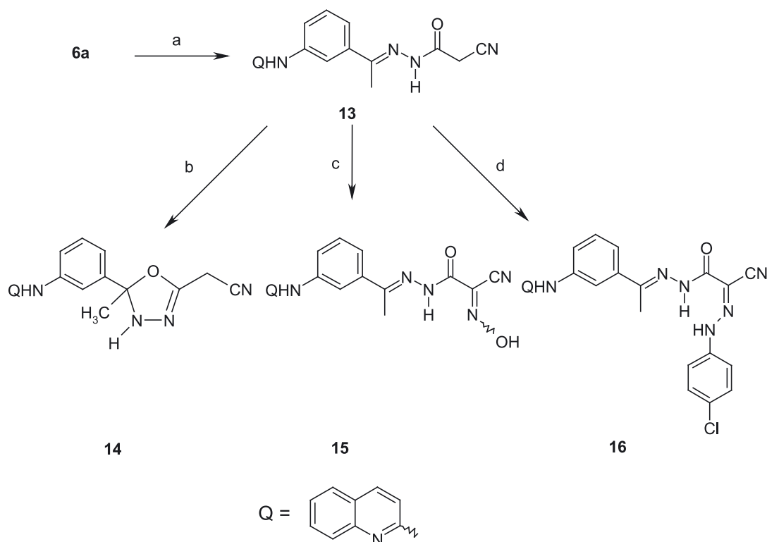
Fig. 3. Reagents and conditions: (a) EtOH, rfx., 75% for 13; (b) \text{Et}_3\text{N} , Dioxane, rfx., 60% for 14; (c) \text{NaNO}_2 , HCl, 0^\circ\text{C} , 70% for 15; (d) p\text{-ClC}_6\text{H}_4\text{N}=\text{NCl} , NaOAc, 0^\circ\text{C} , 65% for 16
