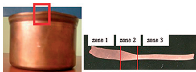
Fig. 3. Drawpiece (left) and its fragment with three strain zones (right): drawn zone – zone 1, transitory zone – zone 2, and after one flow forming operation – zone 3
