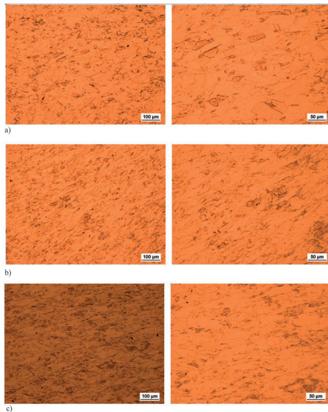
Fig. 9. Structural documentation of sample (as in Fig. 3 and 6 on cross-section) on the sheet surface at magnifications of 10 and 20x, where: a) zone 3 (drawn), b) zone 2 (transitory), c) zone 1 (flow formed)
