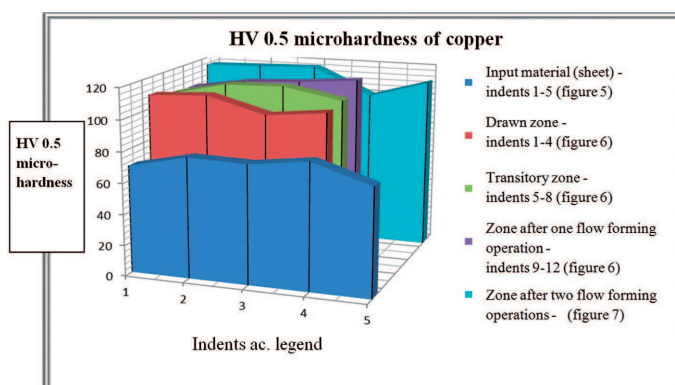
Fig. 8. HV 0.5 microhardness of copper in the form of a sheet, drawpiece, and after one and two operations in the CEFF process
