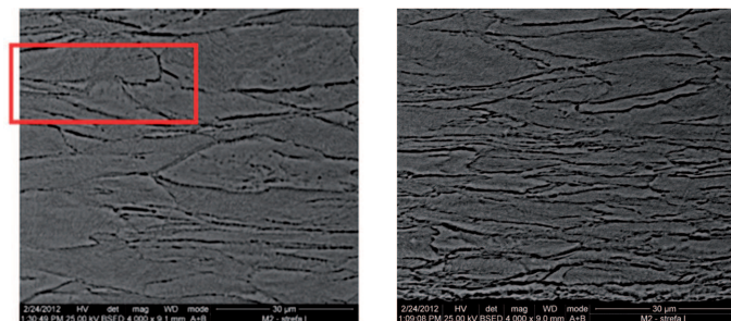
Fig. 11. Indicative images (SEM) of the copper sample collected from zone 1 of sample 2
