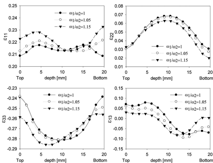
Fig. 12. Strain components \epsilon_{11} , \epsilon_{22} , \epsilon_{33} , \epsilon_{13} vs. distance from the sample surface (depth) after SR and AR with \omega_1/\omega_2 = 1, 1.05 and 1.15 . Entry angle \alpha = 0^\circ (FEM calculation)
