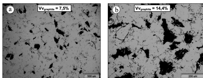
Fig. 5. Microstructure of CuSn10Zn7PTi/C (a), CuSn10Zn7PTi4/C (b) composites
