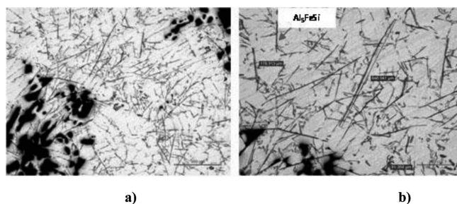
Fig. 3. Microstructure of sample from melt nr. 2 – measurement of iron based phases
