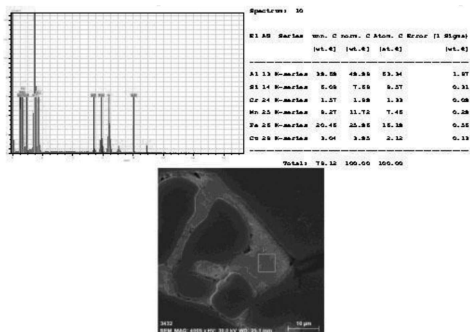
Fig. 6. EDX analysis of coarsen \alpha -phases on sample from melt nr. 3
