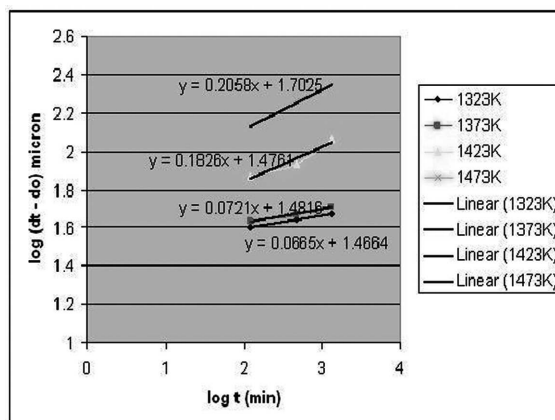
Fig. 4. Graphical plots of \log (D_t - D_0) versus \log t for the superalloy
