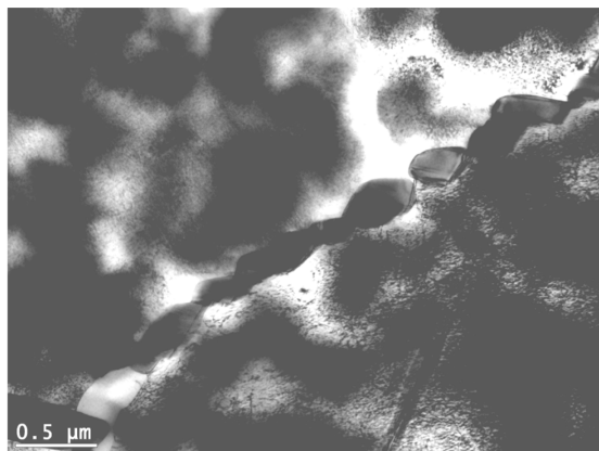
Fig. 6. The example of precipitates with morphology different from the most typical needle-like showed in fig. 5a (x50.000)
