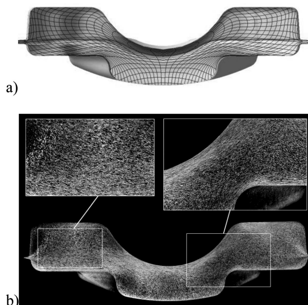
Fig. 4. Flow lines (grain pattern): (a) determined numerically, (b) actual flow lines
