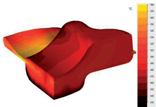
Fig. 7. Distribution of temperature in AA2099 alloy forging
