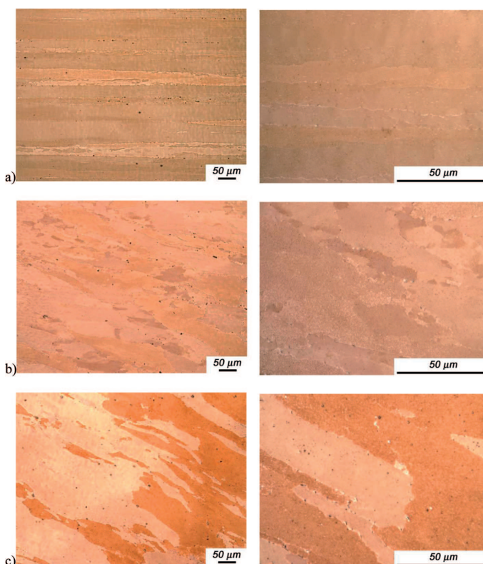
Fig. 10. Microstructure in central part of a forging: (a) longitudinal section (region A), (b) cross section (region B), (c) cross section (region C)
