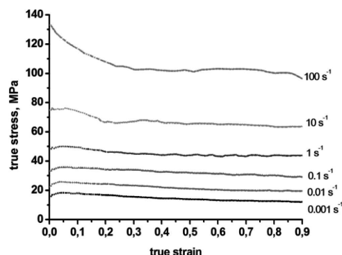
Fig. 2. Stress-strain curves obtained for temperature 500°C and strain rates ranging from 0.001 s -1 to 100 s -1
