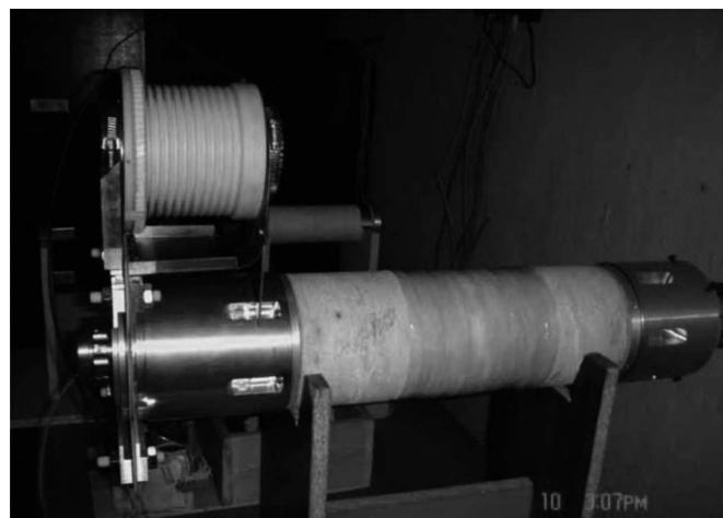
Fig. 5. Magneto-cumulative generator with axisymmetric explosive opening switch
