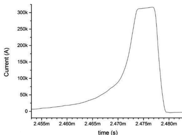
Fig. 6. Axisymmetric EOS performance
