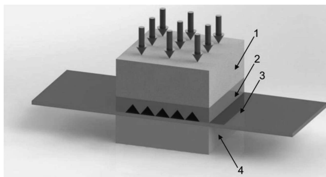
Fig. 1. Scheme of the explosive device for current switching 1 – high explosive; 2 – dielectric jetmaker; 3 – current-carrying conductor; 4 – dielectric barrier
