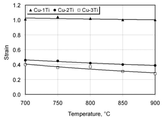
Fig. 13. Change of strain corresponding to the peak flow stress of Cu-Ti alloys deformed at different temperature with strain rate of 10.0 \text{ s}^{-1}
