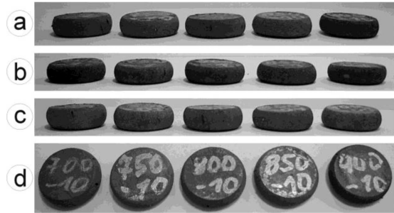
Fig. 5. Appearance of Cu-3Ti alloy specimens after compression at temperature in the range 700\div 900^\circ\text{C} up to a strain of 1.2 (70%) with strain rate of 0.1 (a), 1.0 (b) and 10.0\text{ s}^{-1} (c)
