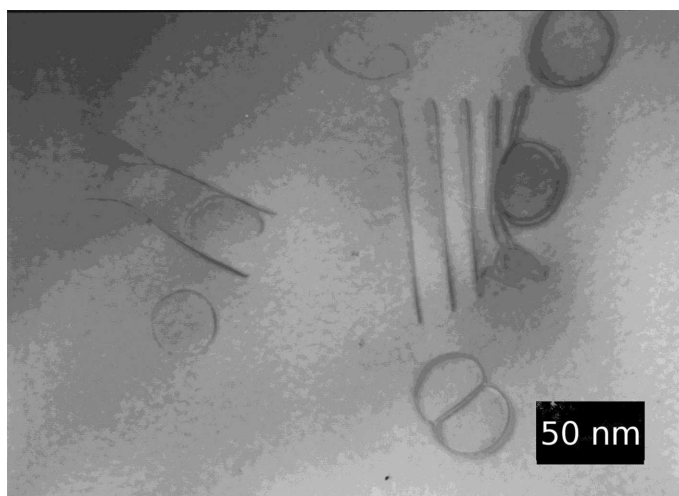
Fig. 1. TEM micrograph of vacancy loops in zinc
