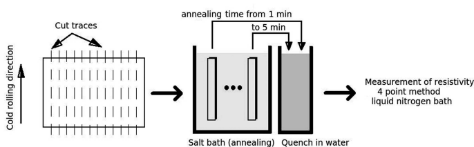
Fig. 2. Preparation of samples: Samples were cut out of the sheet of metal. Next each sample was annealed in salt bath, followed by quenching in water and measurement of resistivity
