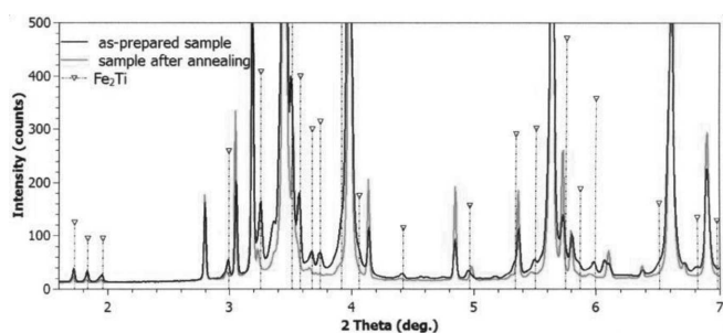
Fig. 7. XRD pattern from the interface area of bimetal 304 SS clad with Ti analyzed using synchrotron (P07) – compared materials without the HT and after the HT
