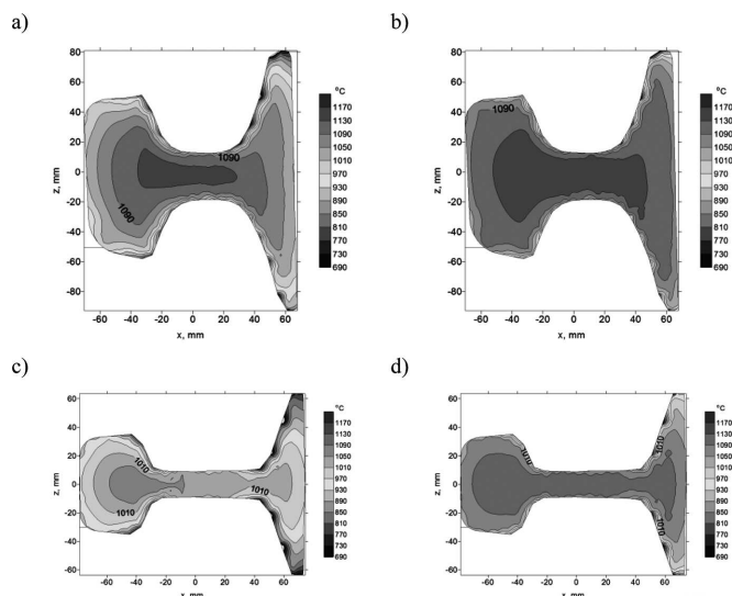
Fig. 8. Temperature field of S49 rail for rolling pass: no. 7- air cooling (a); no 7- aluminum radiation shield (b); no. 10- air cooling (c); no 10- aluminum radiation shield (d)
