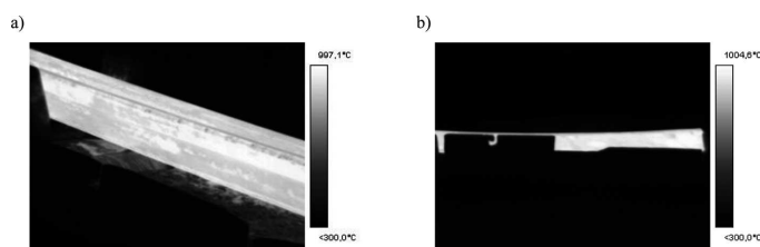
Fig. 3. Thermal photography of S49 rail before (a) and at the end (b) of rolling
