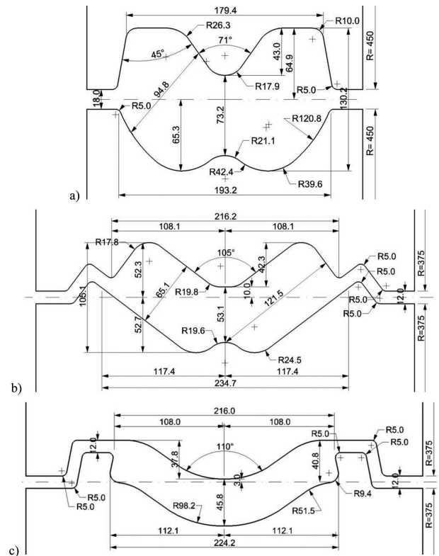
Fig. 1. Shaped grooves for rolling flat bars from a 160×160 mm feedstock: a) slitting groove; b, c) bending grooves
