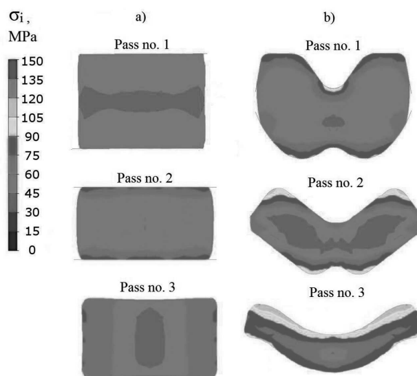
Fig. 4. Distributions of the intensity of stress \sigma_i on a cross section of a strand rolled in three passes in traditional (a) and shaped grooves (b)
