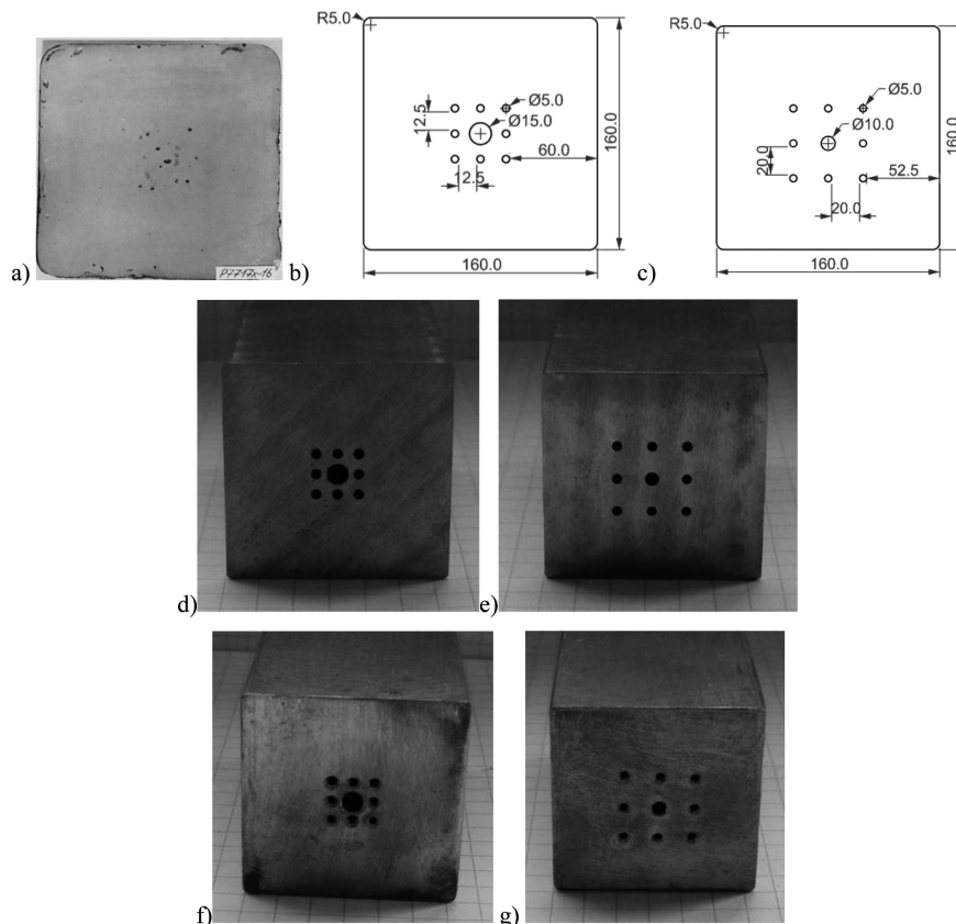
Fig. 2. Images of an ingot with material discontinuities: an actual ingot (a), designed samples with nine holes (b, c), and designed samples for experimental studies: steel (d, e) and lead (f, g)
