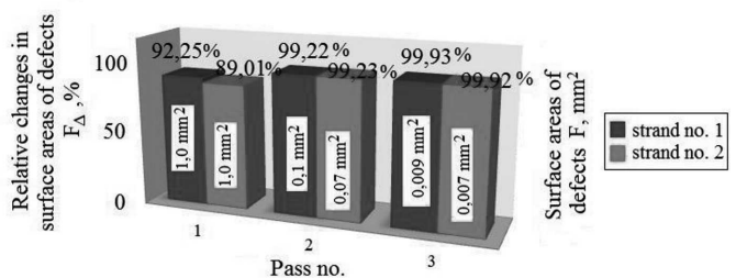
Fig. 10. Relative change in the surface areas of axial defects during rolling of lead samples in three shaped grooves
