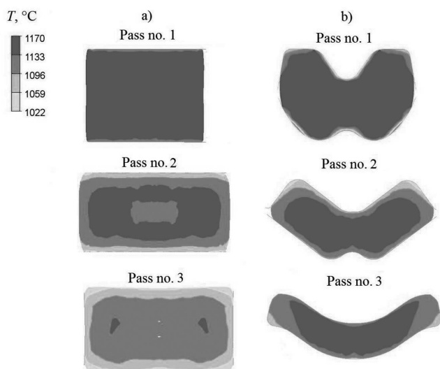
Fig. 3. Temperature T distributions on a cross section of a strand rolled in three passes in traditional (a) and shaped grooves (b)
